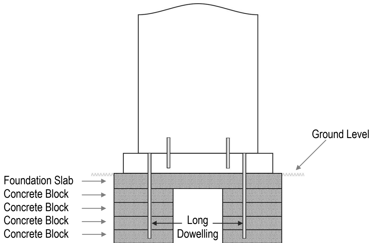
Fig 8 ~ Pillar Foundation Example Using Dowelled Concrete Blocks to form Pillars
