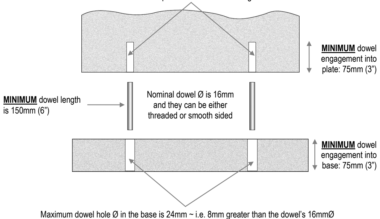
Pic: 4 Granite, Hard Limestone, Marble or Slate Lawn Memorials with an overall height between 900mm (35½") & 1200mm (47½") Minimum plate thickness 75mm (3")
