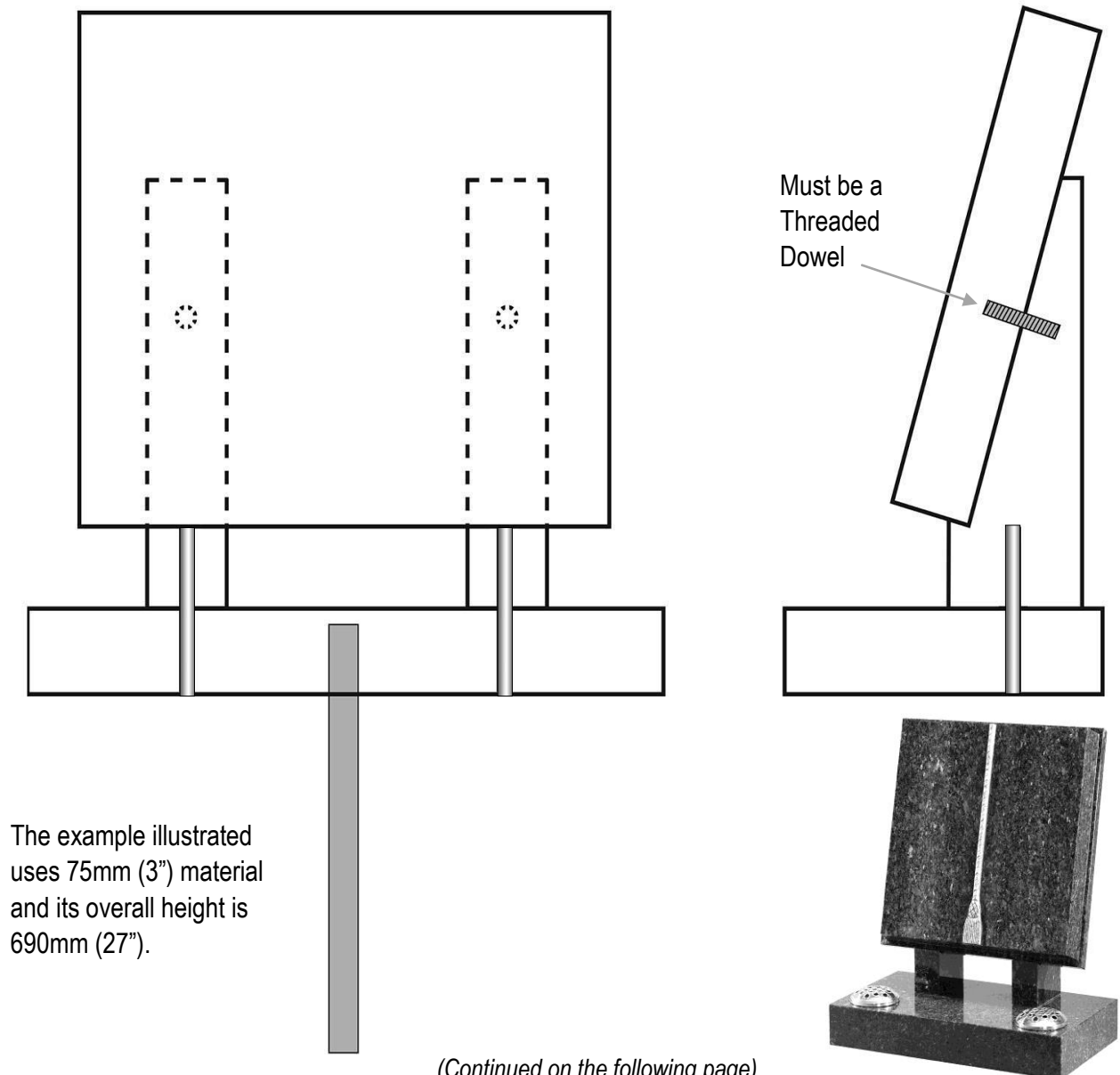
Fig 4 ~ Book Set Memorials
