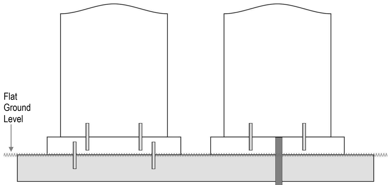
Fig 7 ~ Memorials with Foundations Cast-in-Situ on Sloping Ground
