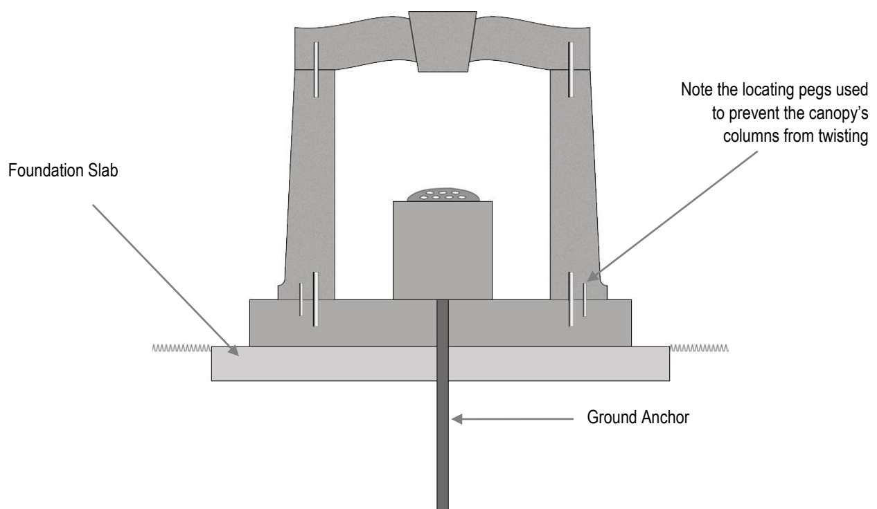
Fig 11 ~ A typical Canopy Set memorial fixed using dowels, locating pegs and ground anchor
