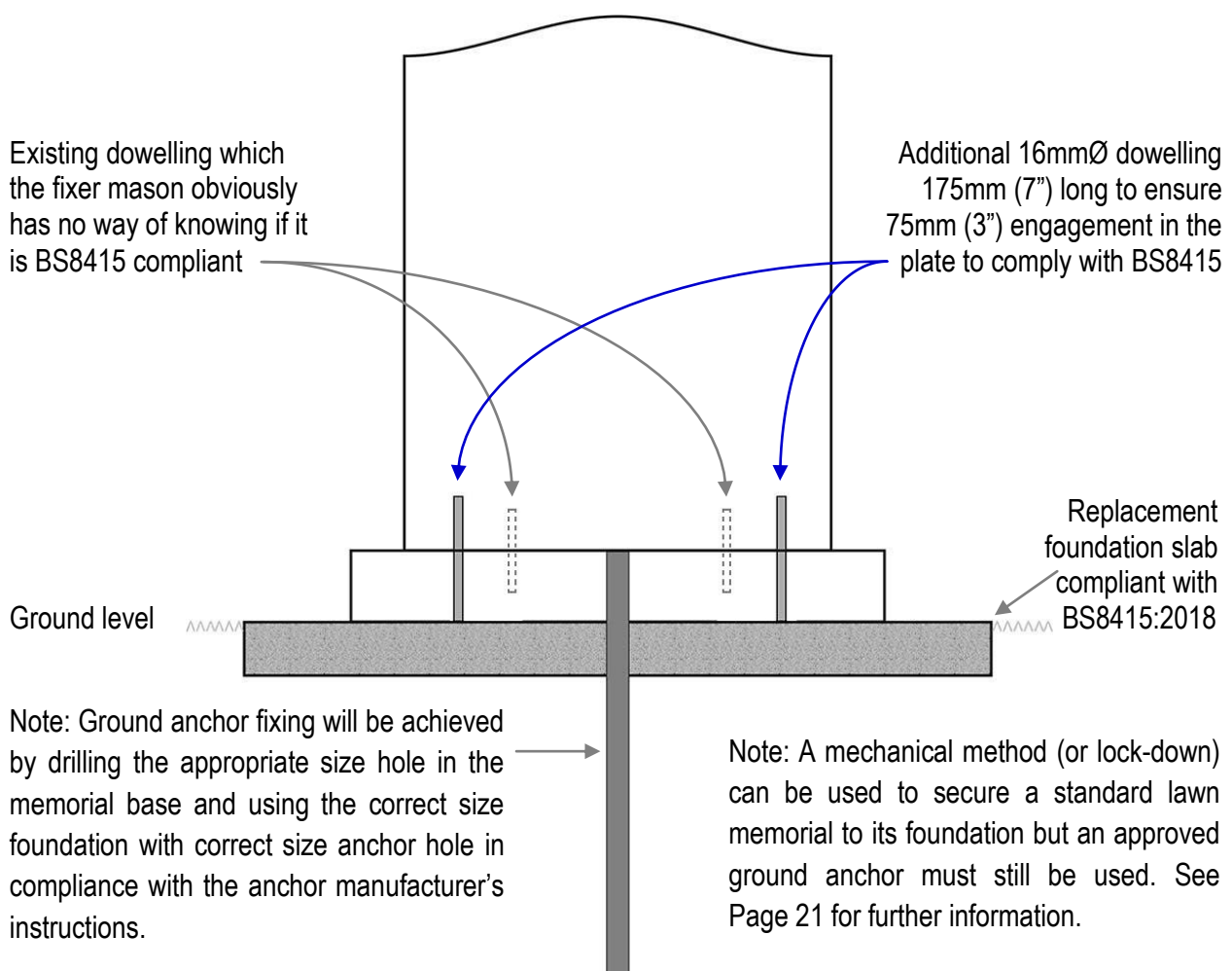
Fig 10 ~ Re-fixed Lawn Memorial ~ Example Shown: Overall Height 900mm (35.5") using 100mm (4") material
