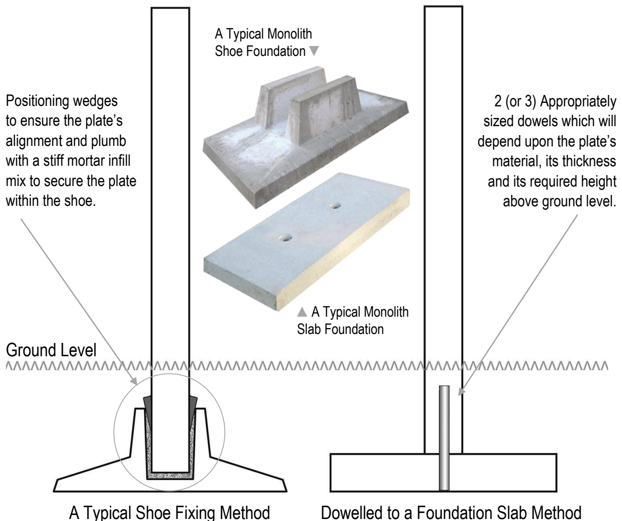
Fig 5 ~ Monolith Memorials ~ there are several recognised methods of installing monolith memorials. Two commonly used methods are shown below.
