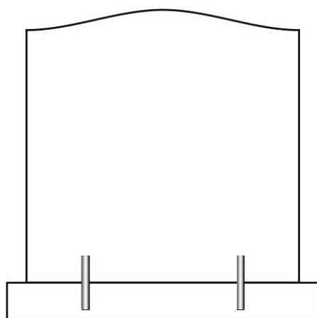
Fig 1 ~ Lawn Memorials Under 625mm (25.5") Minimum material thickness 50mm (2")
