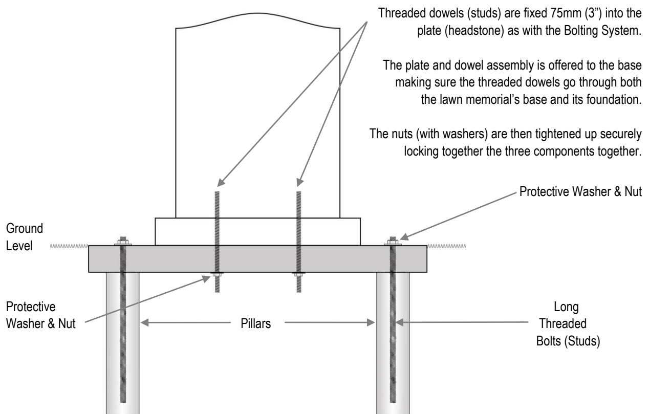
Fig 10 ~ Pillar Foundation using threaded dowels (Studs) and 75mm (3") granite (2'3"x1'9")
